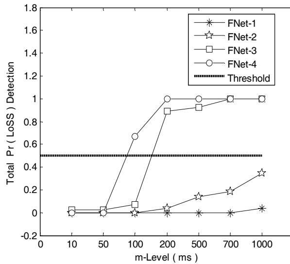
Fig. 5: Probability of continuous LoSS detection.
